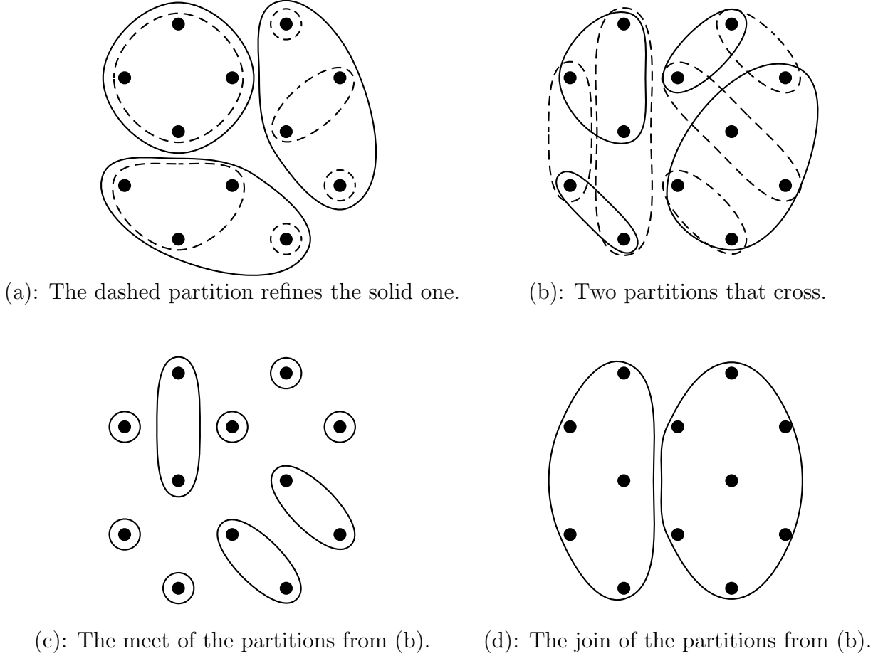
Figure 3.2: Illustrations of some partitions. The black dots are the terminal set R .
