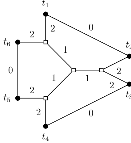
Figure 4.5: This graph shows that \text{OPT}(\mathcal{P}) and \text{OPT}(\mathcal{B}) can be different on 6-preprocessed instances. Dots are terminals and squares are Steiner vertices. Edge costs are shown.
