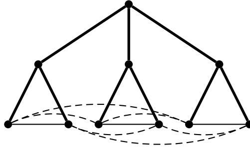
Figure 6.2: An extreme point solution to (\mathcal{F}) . There are 9 edges in the supply graph, shown as thick lines; each has capacity 1. There are 9 demand edges, shown as thin lines; the solid ones have value 1/2 , and the dashed ones have value 1/4 . This is a tight example for Lemma 6.6 because each edge lies on at least three demand paths.
