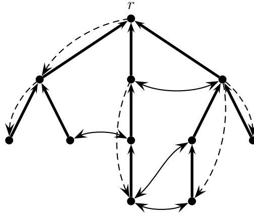
Figure 6.4: An all-ror multicommodity flow instance. The tree graph (V, E) is depicted using thick lines, and the demand edges D are thin. Radial demand edges are dashed and root-using demand edges are solid. The root is r . An arrowhead denotes a positive endpoint, while the remaining endpoints are negative; these signs correspond to the reduction in the proof of Theorem 6.4.
